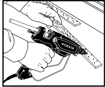
APPLY GLUE TO TACK STRIP IN ONE FOOT LENGTHS
