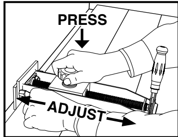
FAST LENGTH ADJUSTMENT AT WALLS
