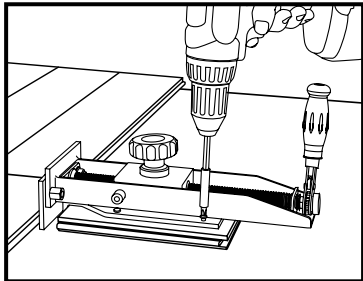
FASTEN TO FLOOR IN MIDDLE OF ROOMS
