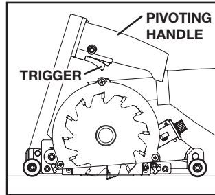
Fig. 10 LOWER PIVOTING HANDLE TO START THE GROOVE
